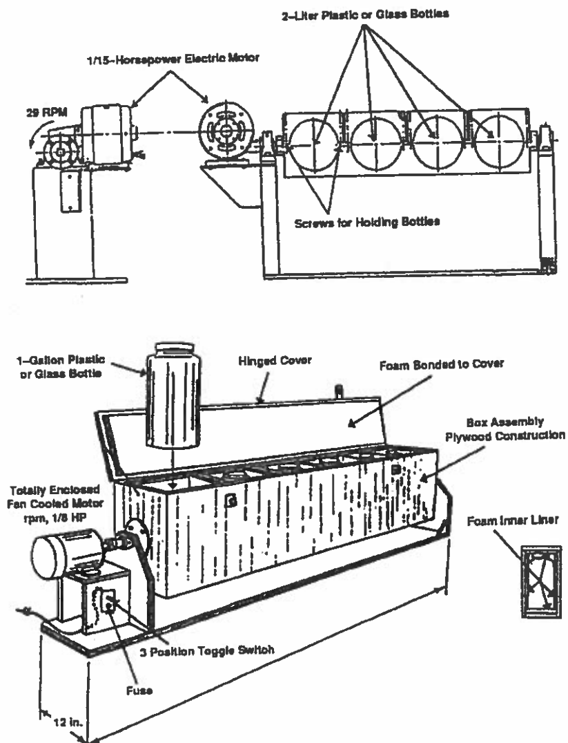
FIG. 1 Extractor
